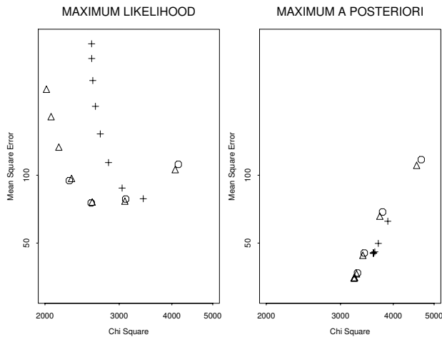
Fig. 9. Convergence of OS-EM and OS-GP. Mean square error versus chi-square at selected iterations: level 1, iterations 16,32,64,128 (○); level 8, iterations 2, 4, 8, ..., 128 (△); level 32, iterations 1, 2, 4, ..., 128 (+).
