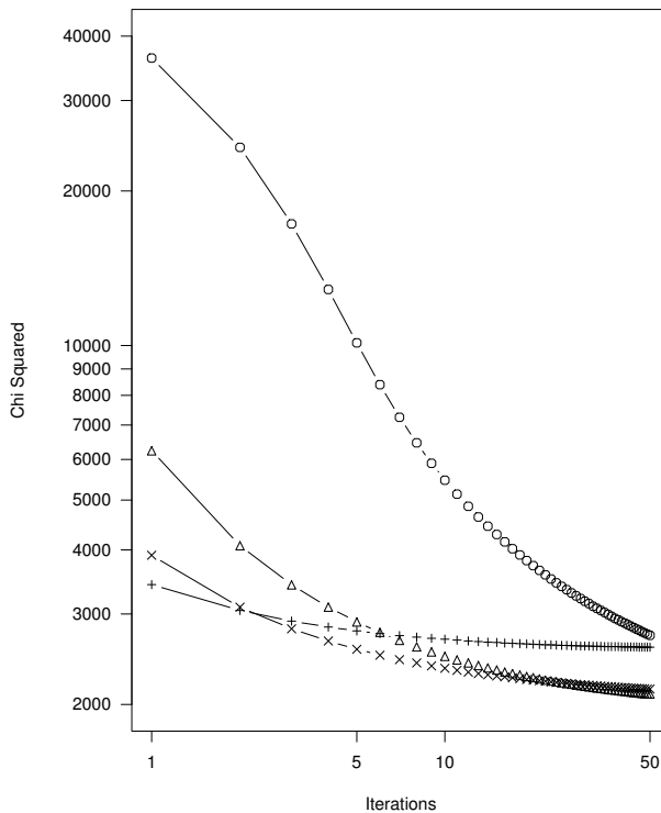
Fig. 5. Chi-square ( G ) vs Iteration (log scale) by OS-EM level: OS-EM level 1 ( \circ ); level 8 ( \Delta ); level 16 ( \times ); level 32 ( + ).
