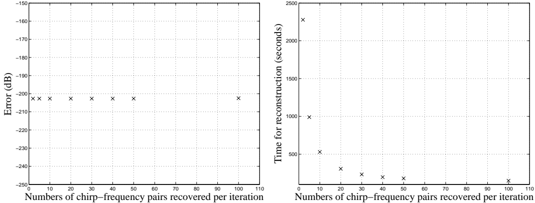
Figure 1. Left: the reconstructed error does not increase when the number of chirp rate-frequency pairs in each iteration increases. Right: Moreover, when the number of chirp rate-frequency pairs in each iteration increases, the reconstructed time decreases rapidly.
