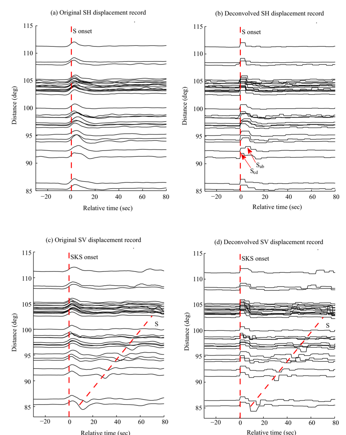
Figure 5. Original and deconvolved SH and SV trace. Broadening between 90 and 98 deg is consistent with the D'' related S_{ab} and S_{cd}
