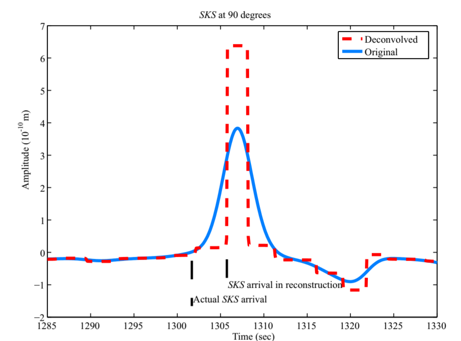
Figure 4. Deconvolved synthetic SKS
