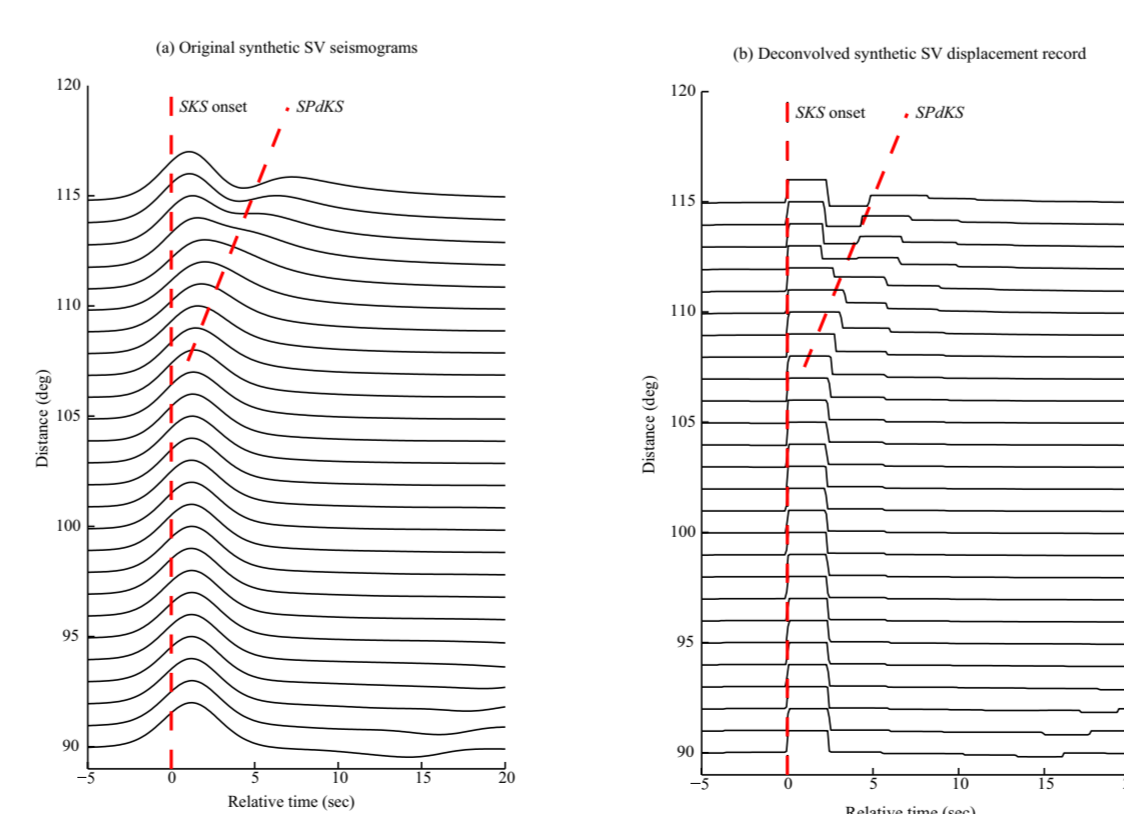
Figure 3. Original and deconvolved SV trace, aligned at edges in (b)
