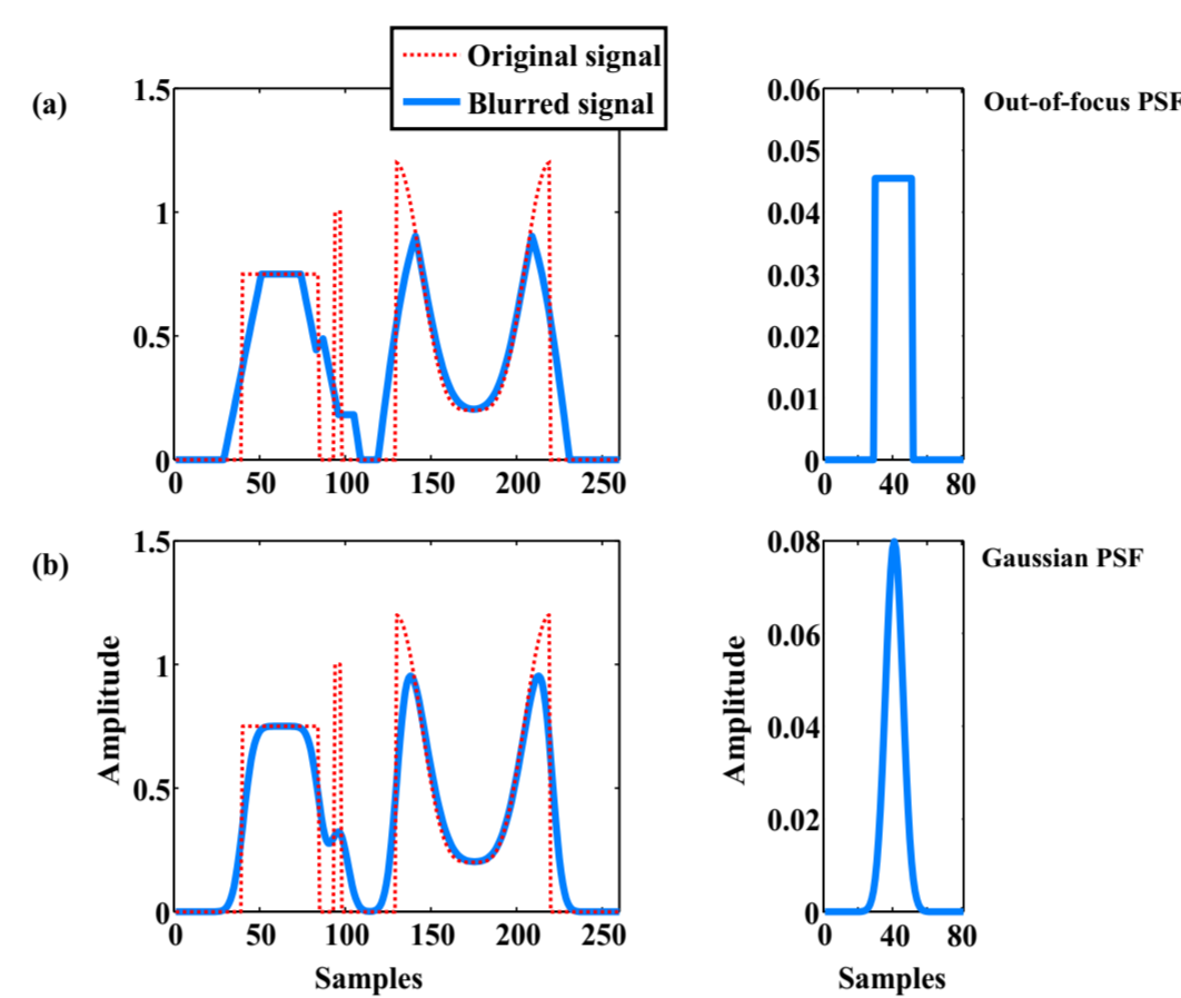
Figure 2. Blurring by different PSFs.
