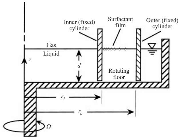
FIGURE 1. Schematic of the flow apparatus.
