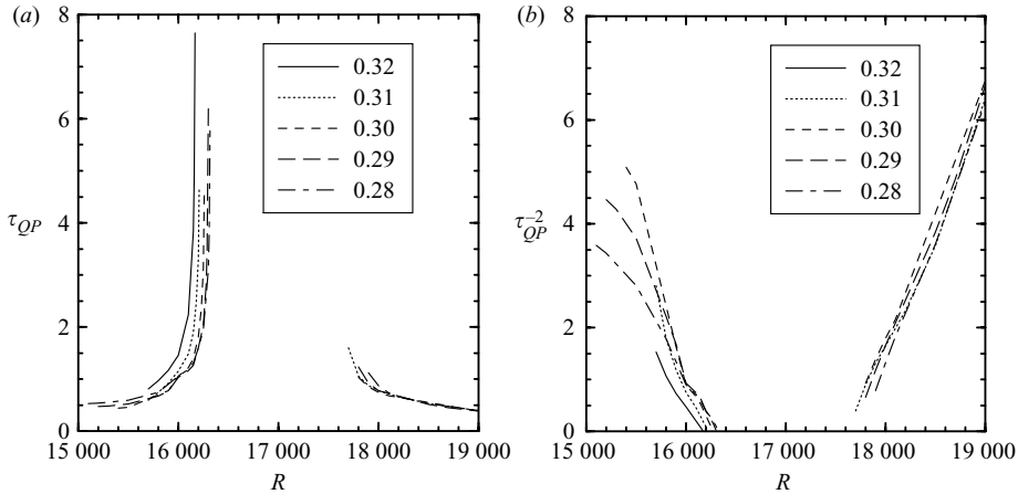
FIGURE 19. (a) Variation of the modulation period \tau_{QP} with R for various F as indicated; in (b) the data is plotted as \tau_{QP}^{-2} , showing the typical scaling of the frequency in the neighbourhood of SNIC bifurcations.
