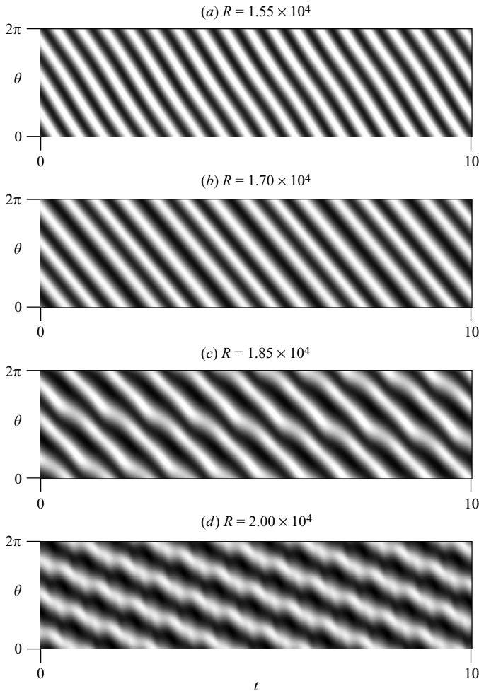
FIGURE 20. Space–time diagram of \Theta(r=1, z=0) for the mixed-mode solutions at (a) R=1.55 \times 10^4 ( QP ), (b) R=1.70 \times 10^4 ( L_{13} ), (c) R=1.85 \times 10^4 ( QP ) and (d) R=2.00 \times 10^4 ( QP ), all at F=0.30 . The grey scales are from cold (black) to hot (white) in the range \Theta \in [-0.3, 0] . The accompanying movies in the online version are animations of these three states, showing contour plots \Theta in a horizontal cross-section at mid-height.
