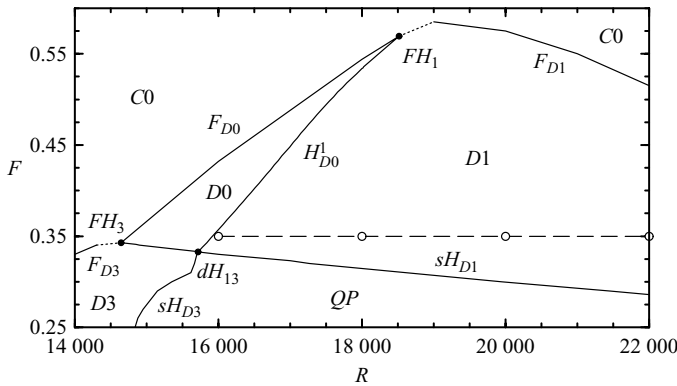
FIGURE 12. Bifurcations of the rotating wave D1 , showing the Hopf bifurcation curve H^1_{D0} where D1 is born, and the fold curve F_{D1} and the secondary Hopf curve sH_{D1} where D1 becomes unstable. These curves meet at the codimension-two points FH_1 and dH_{13} . The symbols on the dashed line are the loci of the D1 states shown in figure 13.
