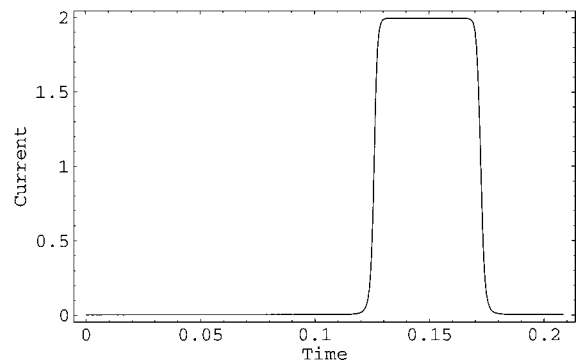
Figure 4. Outflow current in picoamperes for V = -10 millivolts, Gauss' law and Poisson's equation cases, vs. time in millisecond.
