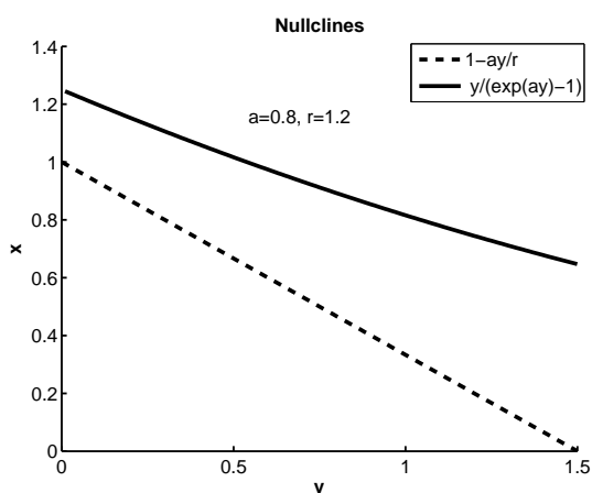
(a) No interior equilibrium: r = 1.2, a = 0.8
