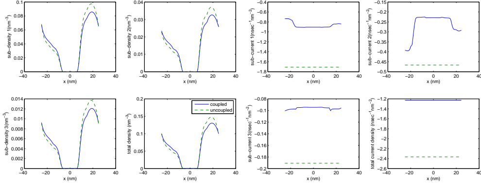
FIG. 6.4. Comparison between the coupled and uncoupled case for three sub-bands. Left 4 Panels: particle densities. Right 4 panels: current densities. Solid lines: with coupling, Dashed lines: without coupling. Second bottom panel from left: total particle density. Fourth bottom panel from left: total current density.
