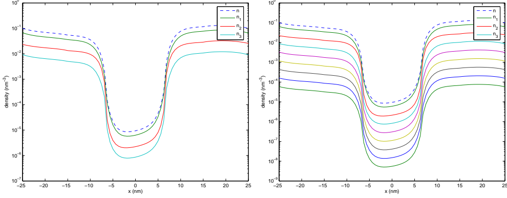
FIG. 6.3. Sub-band densities n_\alpha(x) and total particle density (dashed line) using three (left panel) and eight (right panel) expansion terms.
