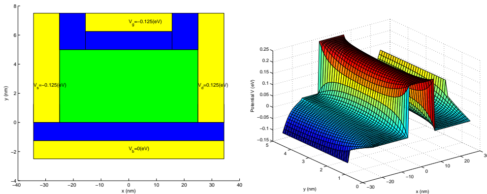
FIG. 6.1. Left Panel: Schematic, green=simulation domain, blue= metal contacts, yellow=insulating oxide. Right Panel: Potential V from the Boltzmann model (6.1).
