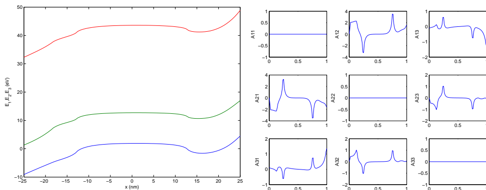
FIG. 6.2. Left Panel: Band energies E_\alpha(x) . Right Panel: Coupling coefficients A_{\alpha\beta}(x) for the first three terms in the sub-band expansion.
