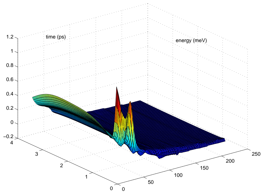
Figure 6: Filtered solution of the Levinson equation.
