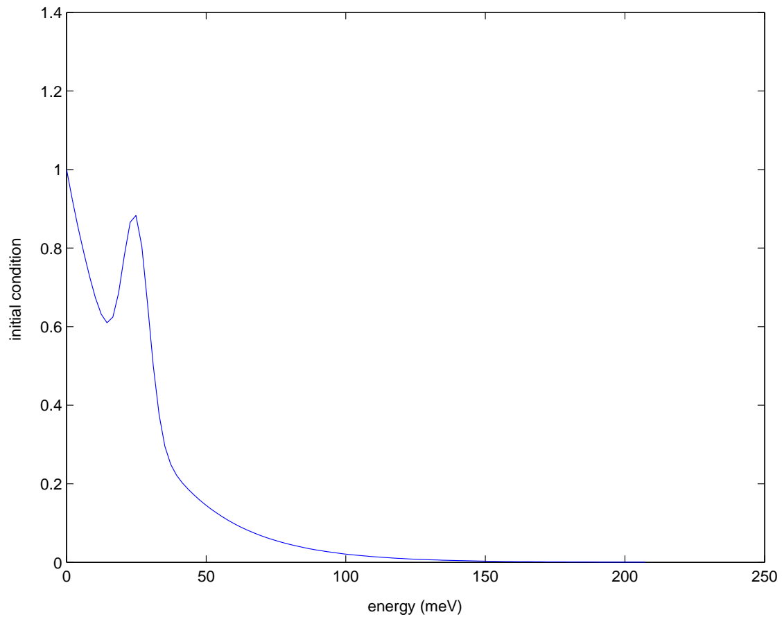
Figure 4: Initial condition for the Levinson equation.
