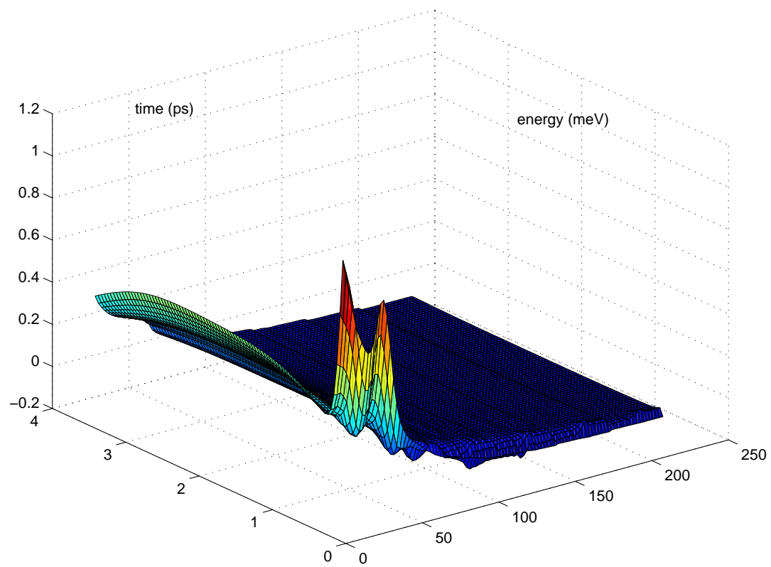
Figure 7: Approximate Solution of the Levinson equation.
