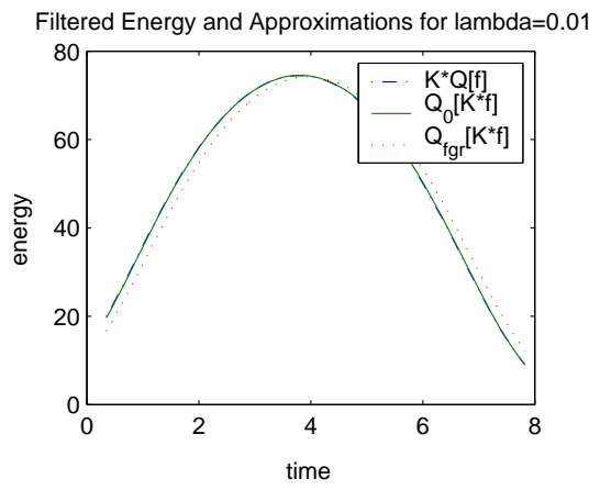
Figure 3: Comparison of Energies.
