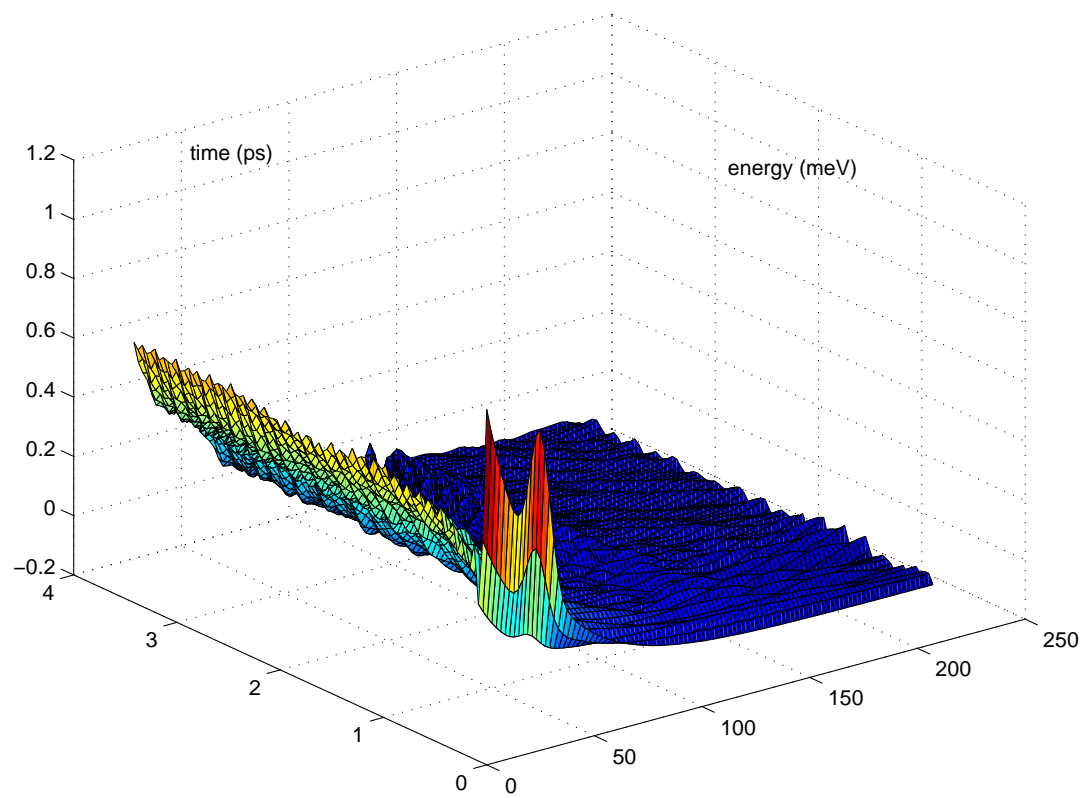
Figure 5: Solution of the Levinson equation.
