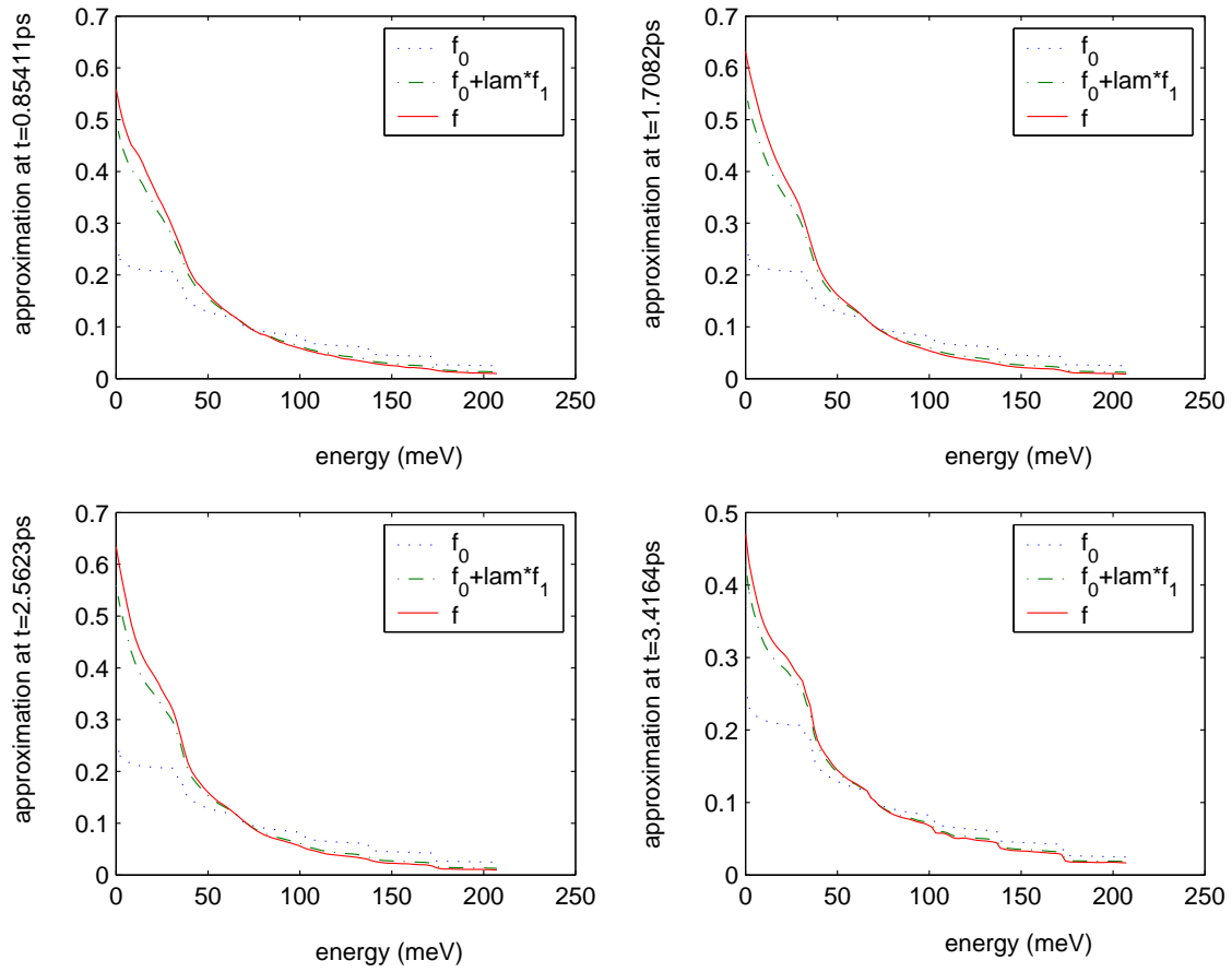
Figure 8: Snapshots of the solution and its approximations.
